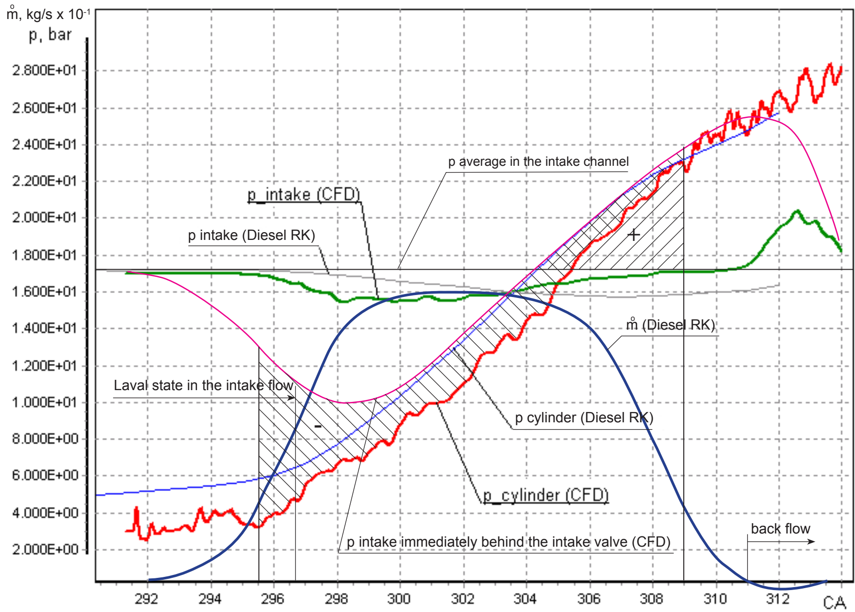
Intake flow of the Z-engine at 3600 rpm, full load
